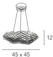
Matrix 1370/S1L 1 x max 50W GU10 230V
