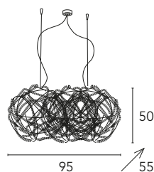
Caleidos 1330/S2L 2 x max 200W R7S 118mm 230V
