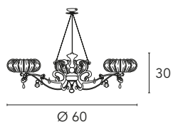
Dream 1306/L3L 3 x max 60W G9 230V
