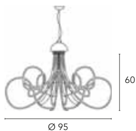
Chic 2010/S8L 8 x max 40W G9 230V
