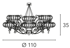
Dream 1306/L8L 8 x max 60W G9 230V
