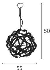
Caleidos 1330/S1L 1 x max 200W R7S 118mm 230V
